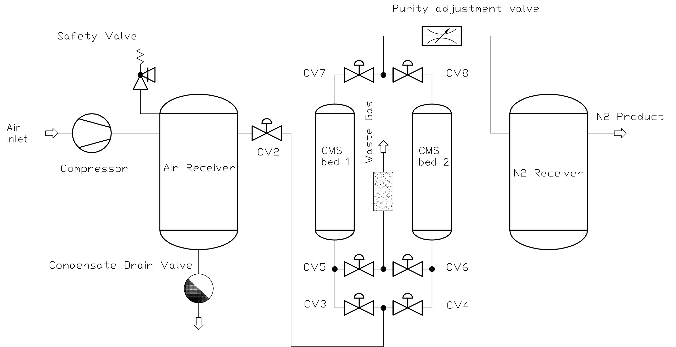
Simplified Schematic of Pressure Swing Adsorption (PSA)
